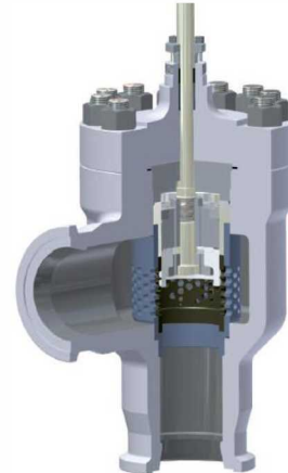
Figure 4 : Valve with HF-LCV trim
